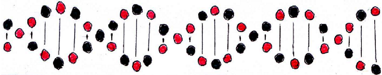
Fig. 1. A single magnetic line of force. The electrons are shown in red and the positrons are shown in black. The double helix is rotating about its axis with a circumferential speed equal to the speed of light, and the rotation axis represents the magnetic field vector \mathbf{H} .
